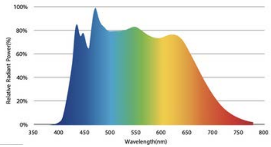
Spectrum curve @5600K
